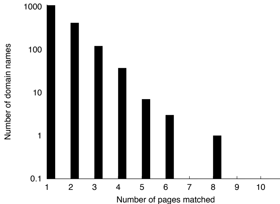
Fig. 5: Number of domain names with x pages matched.
