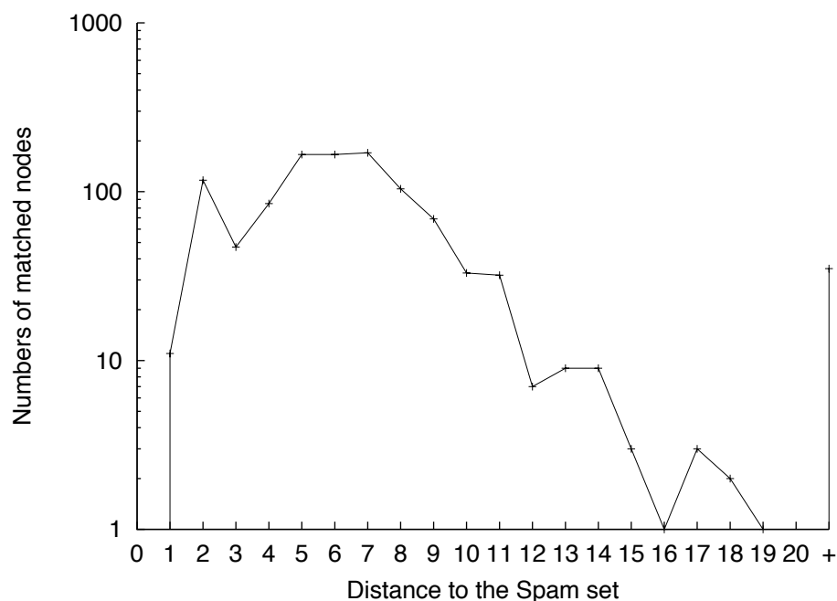
Fig. 3: Distances to the spam set for the nonspam matches.
