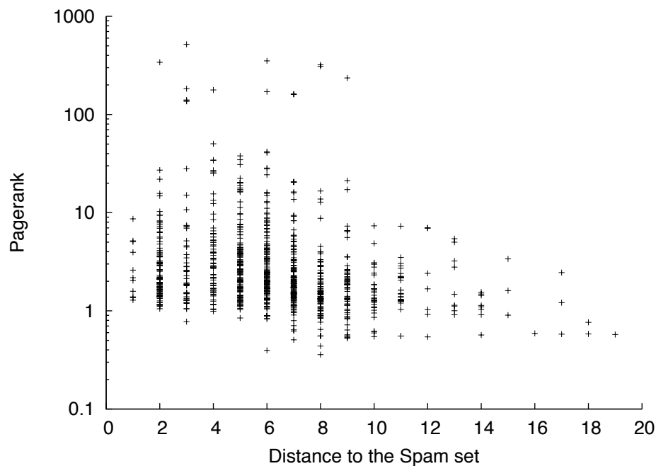
Fig. 4: Pageranks of the nonspam matches w.r.t. their distance to spam set.
